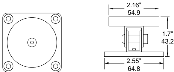
Armature Plate with Mount for Rofu Door Holder Magnets
