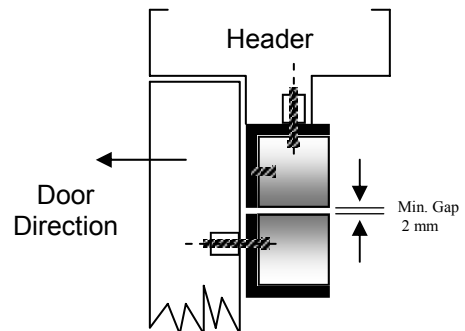
ROFU #21054, Housing with L-Brackets for ROFU 8035 Mini Shear Lock
